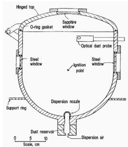
Figure 1: 20-Liter Explosibility Test Chamber
